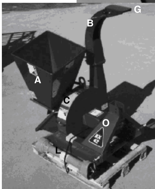
Fig. 10 PRINCIPLE COMPONENTS
